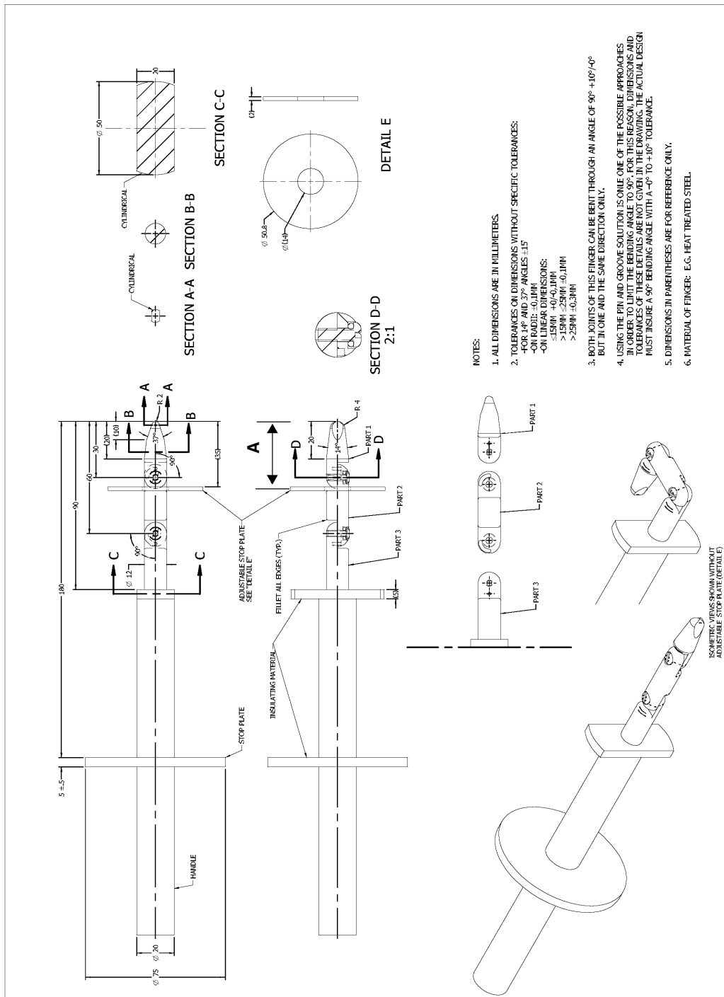
Figure 7-4 Test Finger
