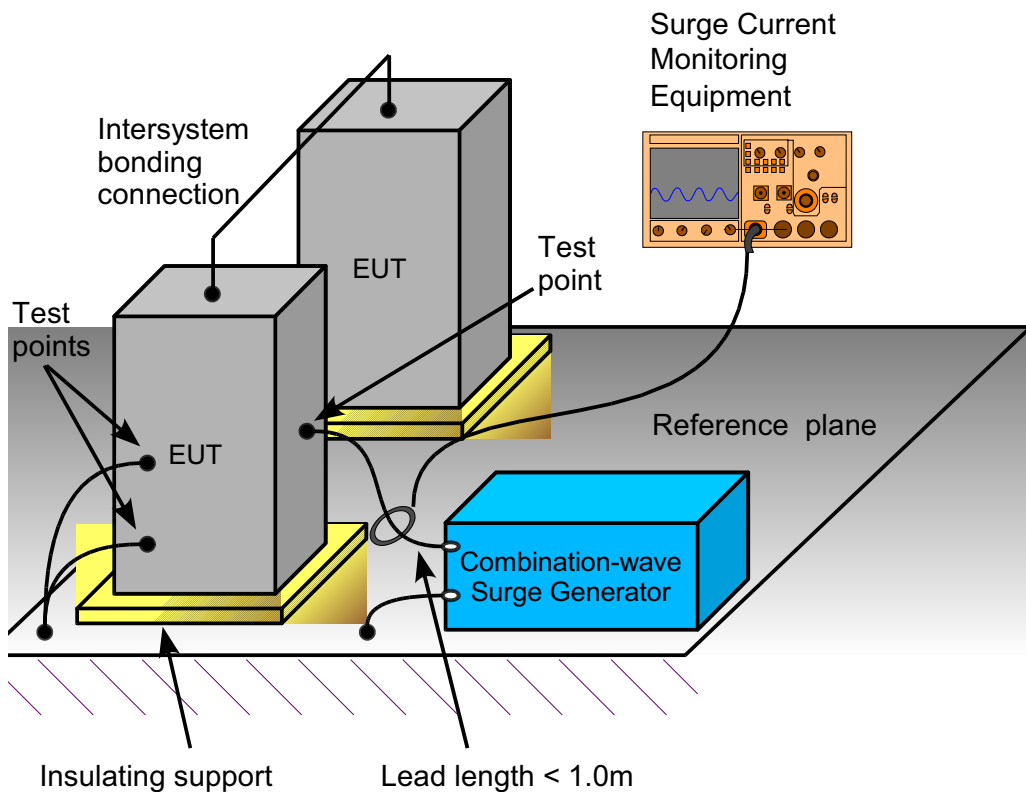
Figure 9-5 Laboratory Configuration for the Frame Surge Test
