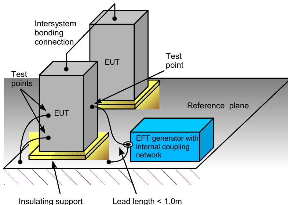
Figure 9-3 Configuration of the Proposed EFT Frame Test
